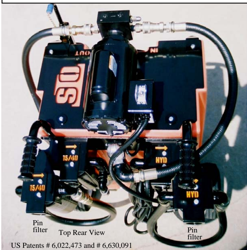
Four filter assemblies with gauges, labeled for any oils you wish Two of which are interchangeable pin filter assemblies
